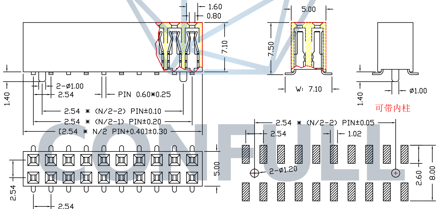
PCB LAYOUT
